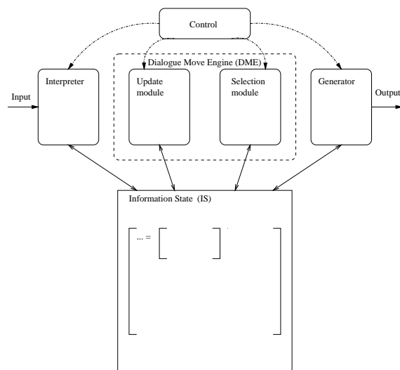
Figure 1: TrindiKit Architecture
